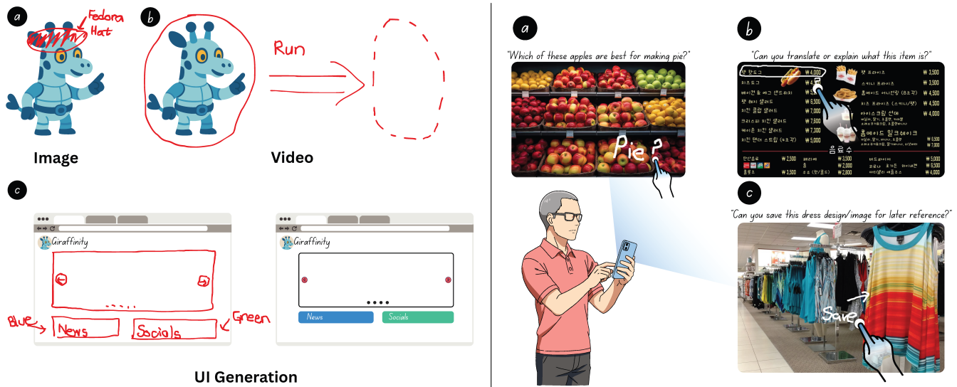
Figure 15: Sample use cases of using annotations: Left: editing and refining generative content, including (a) refining image generation, (b) making action flows for video generation, and (c) creating and editing user interfaces. Right: interacting with a phone using on-screen annotations and form complex queries, such as (a) which apples are best for apple pies, (b) translation, and (c) saving an item for later reference. All sample queries are sourced from ChatGPT and paired with the corresponding image.
