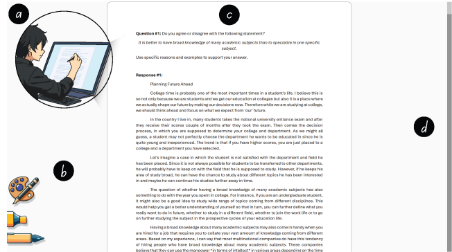
Figure 4: (a) Illustration of a user annotating on the Microsoft Surface Studio desktop. Prototype interface of AnnotateGPT comprises three components: (b) the toolbar (from top to bottom: colour palette, highlighter, and pen), (c) the document, and (d) the specialized scrollbar.
