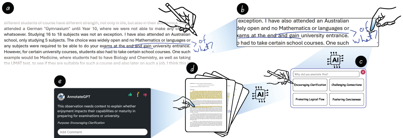
Figure 1: A high-level overview of the interaction design of AnnotateGPT. (a) The user manually annotates the document. (b) Tapping on an annotation will activate the assistant. (c) The assistant will guess the purpose of the annotation. (d) Selecting a purpose will prompt the assistant to provide further annotations (yellow highlights) based on the selected purpose. (e) Users can read, verify and continue the feedback.
