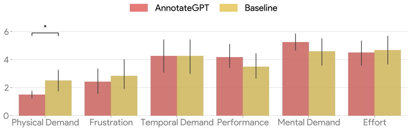
Figure 17: Plot representing the TLX scores across AnnotateGPT and baseline. Asterisk depict significant difference ( p < 0.05 ).
